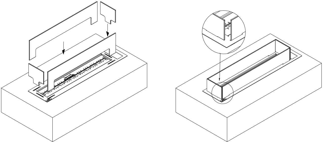
Fig. 4 – Glass installation
