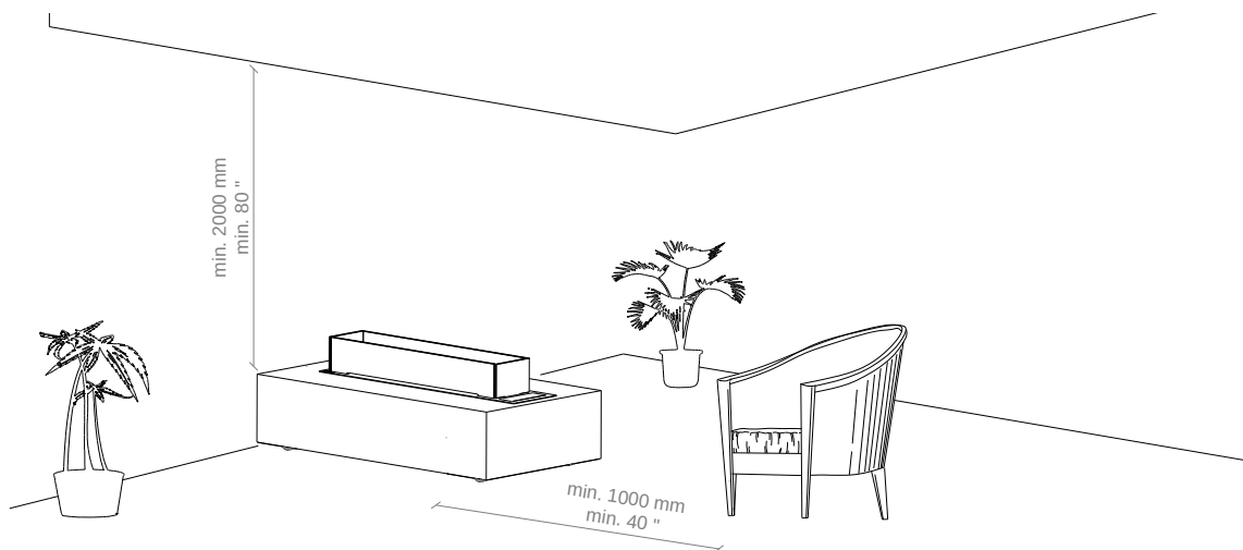
Fig. 1: Minimum distance to flammable materials
