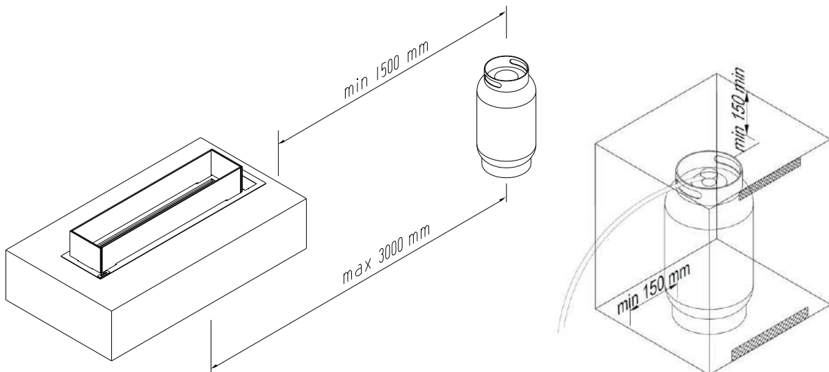
Fig. 5 – Gas cylinder distance and housing for gas cylinder
