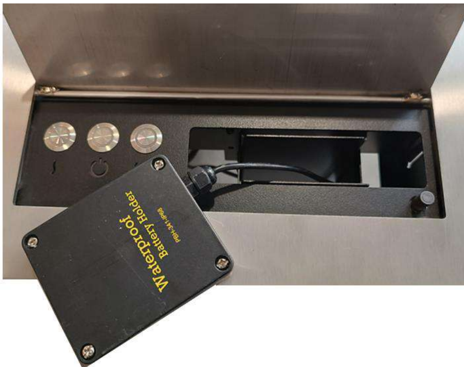
Fig. 9 – Removing of the battery container
