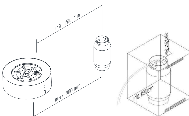
Fig. 4 – Gas cylinder distnace
