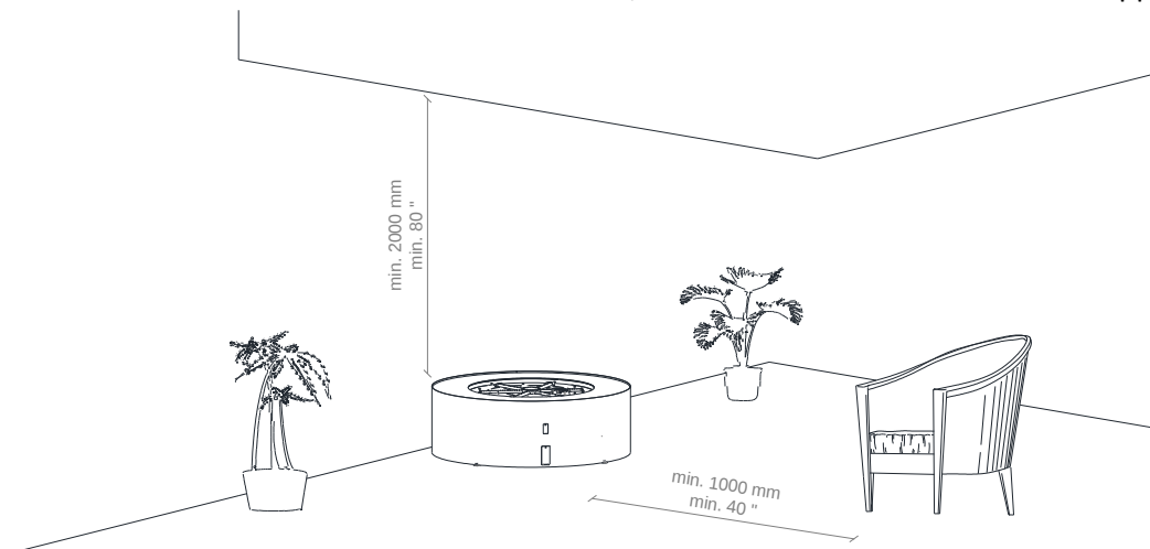
Fig. 1: Minimum distance to flammable materials
