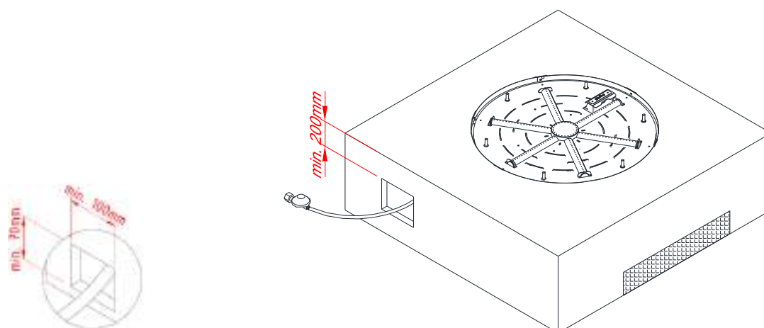
Fig 4 – Gas connection
